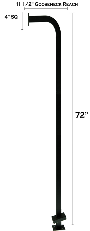
Pad Mount - Truck Height K-18-012
